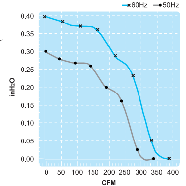
(Axial Fan)
