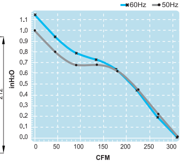
(Duct Fan)
