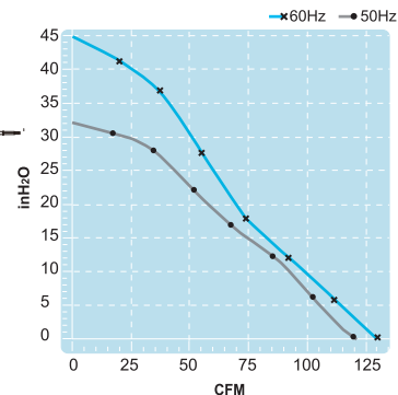
(Blower Fan)
