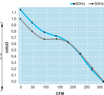
(Duct Fan)
